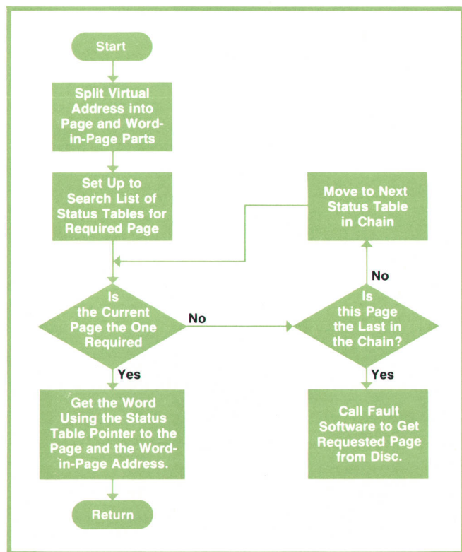
Fig. 2. At a given time, the main computer store contains a number of 2^N -word pages from the virtual memory along with a small status table for each of these pages. The status tables are arranged in a list with the table for the most recently accessed page at the top of the list.
