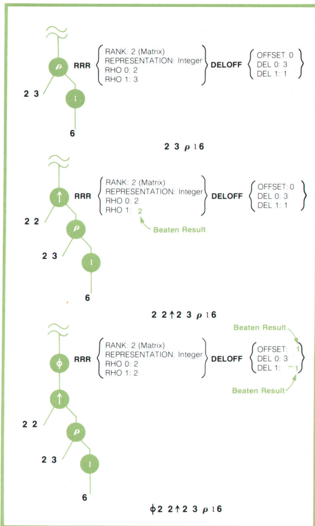
Fig. 6. When evaluation is finally required, beating, or the application of the subscript calculus to a deferred expression, may produce results by description manipulation alone. Here TAKE (↑) and REVERSAL (ϕ) are applied to descriptions for a simple expression. The dragalong (see Fig. 5) and beating strategies can significantly reduce the computation and storage required in the evaluation of an expression.
